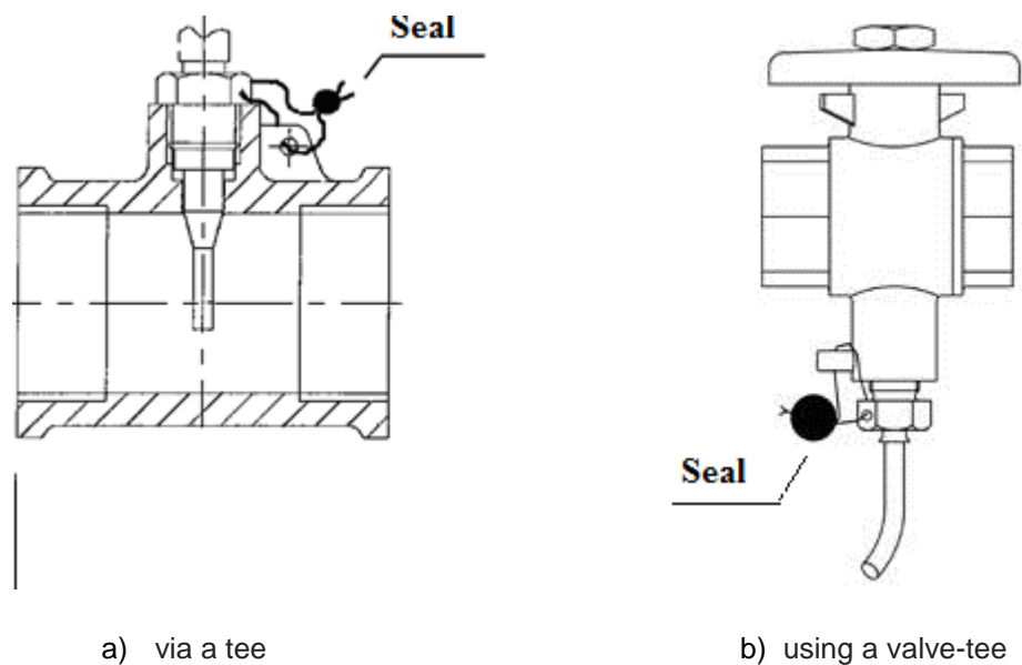
Fig.F4. Installation recommendations for temperature sensors type DS
