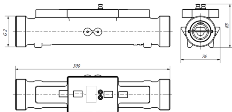
Fig. E6. Dimensions of flow sensors G2" , L=300 mm
