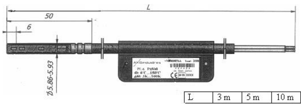
Temperature sensors with permanently connected signal leads L- signal leads length
